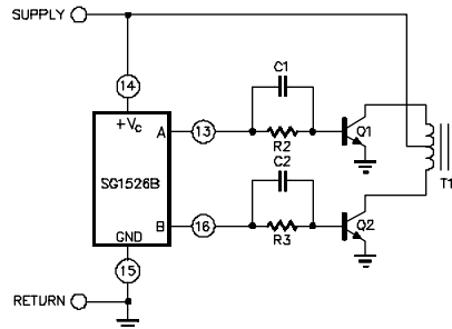
FIGURE 26. PUSH-PULL CONFIGURATION
