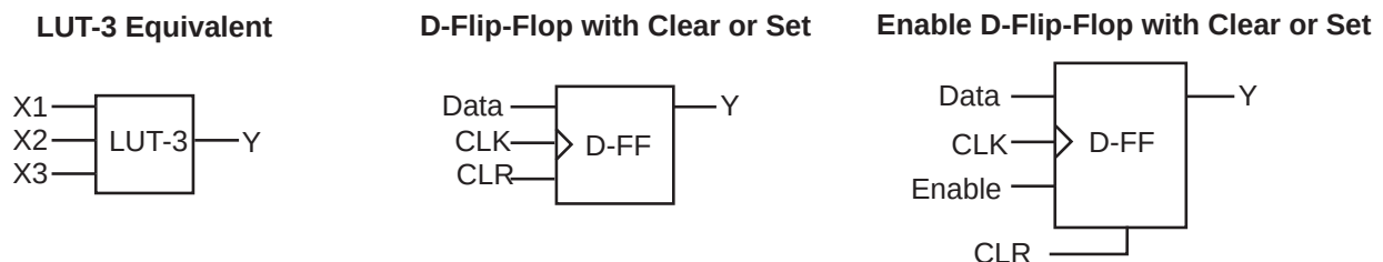
Figure 1-4 • VersaTile Configurations
