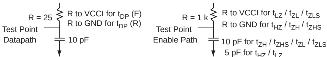
Figure 2-15 • AC Loading
