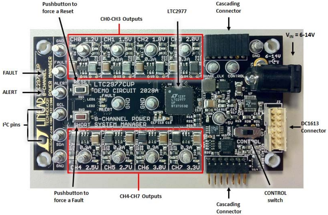
Figure 3. DC2028A Top Side Details
