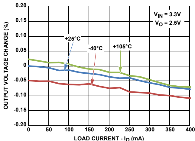
FIGURE 4. LOAD REGULATION
