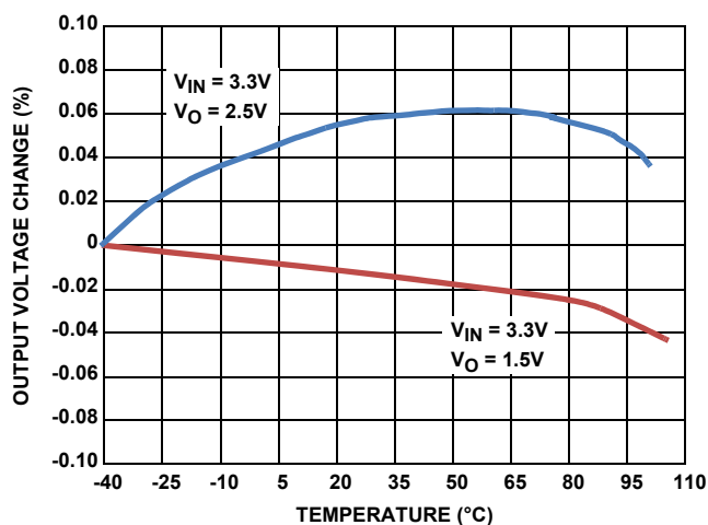
FIGURE 5. OUTPUT VOLTAGE CHANGE vs TEMPERATURE
