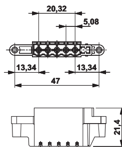
Dimensioned drawing
