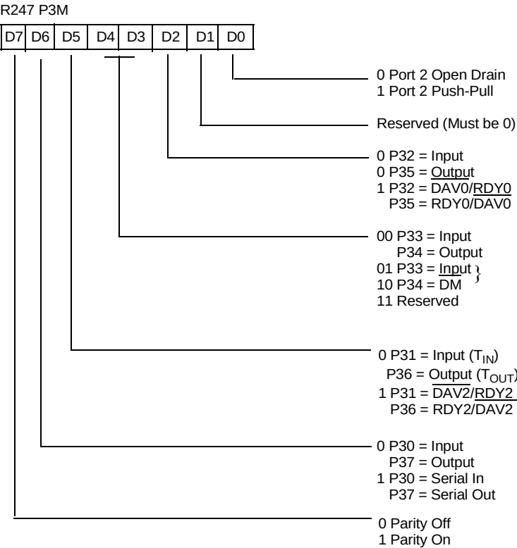
Figure 28. Port 3 Mode Register (F7h: Write Only)
