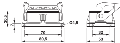
Panel cutout
