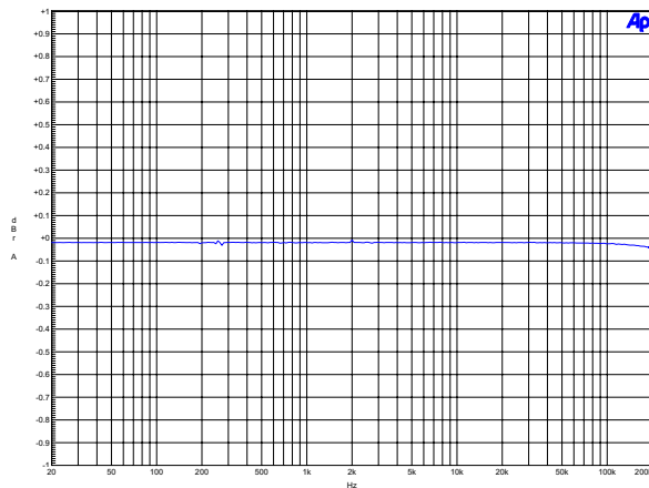
Figure 3. Frequency Response
