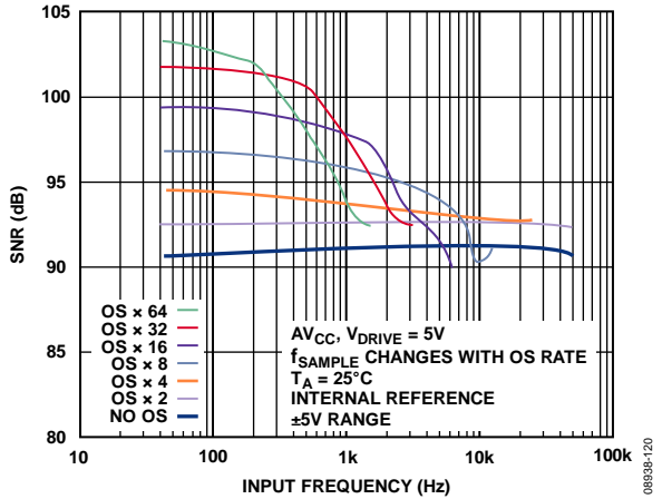
Figure 20. SNR vs. Input Frequency for Different Oversampling Rates, \pm 5V Range
