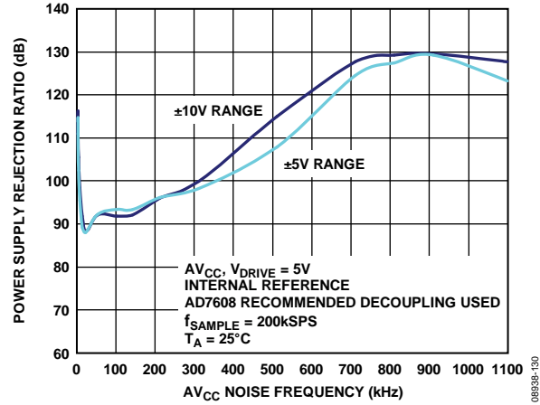
Figure 30. PSRR
