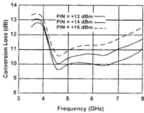
Conversion Loss
