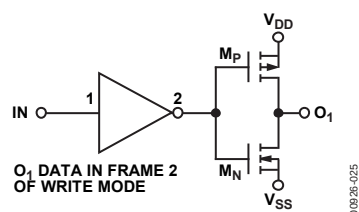
Figure 34. Output Stage of Logic Output, O_1
