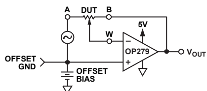
Figure 26. Inverting Gain
