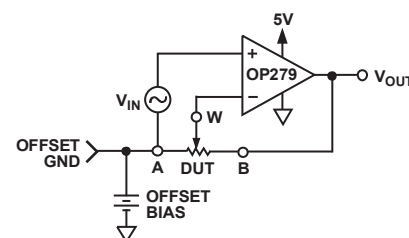
Figure 27. Noninverting Gain
