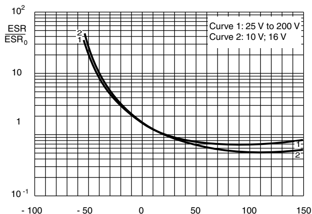
Case \varnothing D \times L = 6.5 \text{ mm} \times 18 \text{ mm} to 15 \text{ mm} \times 30 \text{ mm} ESR 0 = Typical at 20 °C, 100 Hz
