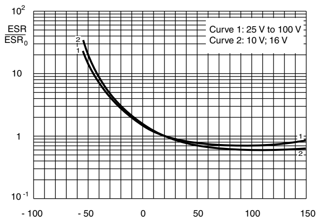
Case \varnothing D \times L = 18 \text{ mm} \times 30 \text{ mm} to 21 \text{ mm} \times 38 \text{ mm} ESR 0 = Typical at 20 °C, 100 Hz
