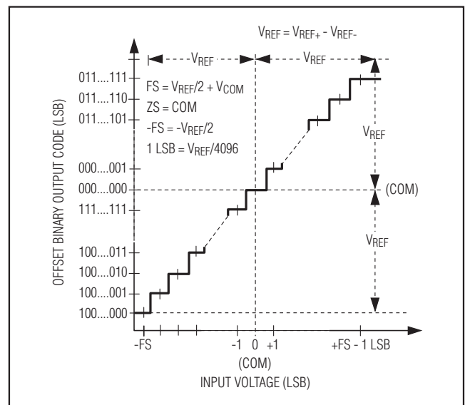
Figure 4. Bipolar Transfer Function—Full Scale (±FS) = ±VREF/2
