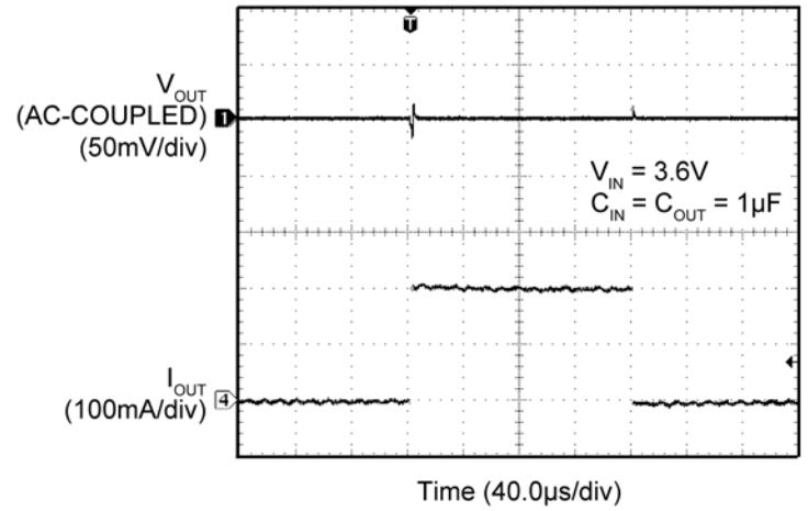
Load Transient (0mA to 200mA)
