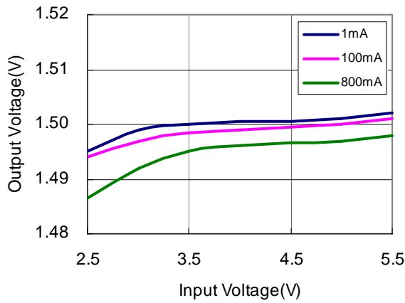
RP501K151x(PWM fixed)
