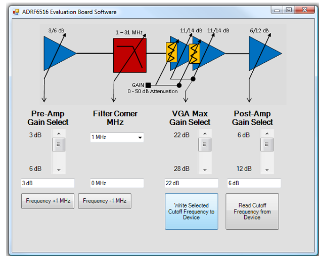
Figure 57. ADRF6516 Evaluation Software
