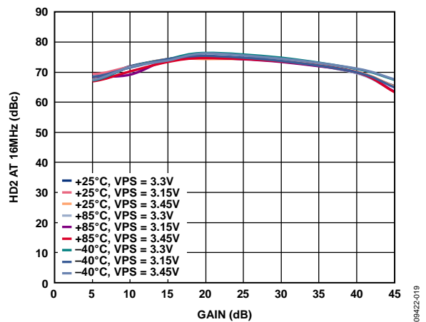
Figure 19. HD2 vs. Gain over Supply and Temperature (Bandwidth Setting = 31 MHz, 1.5 V p-p, 8 MHz CW Fundamental Output)
