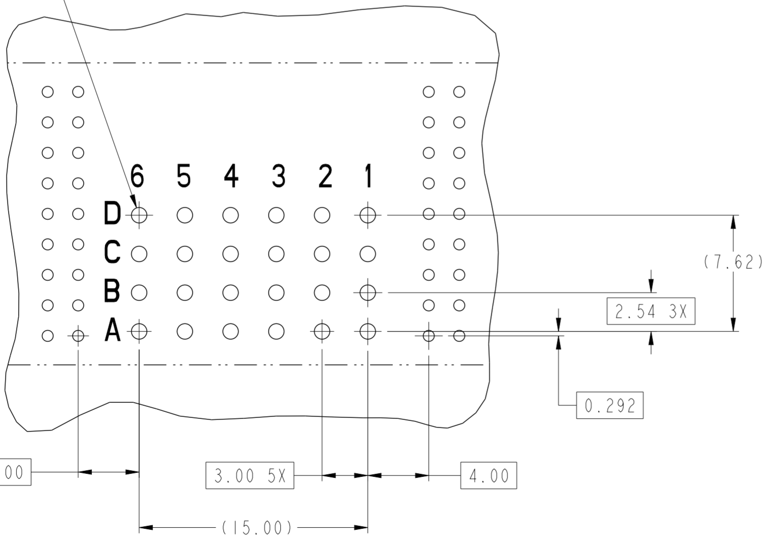
DETAIL E SCALE 4:1
