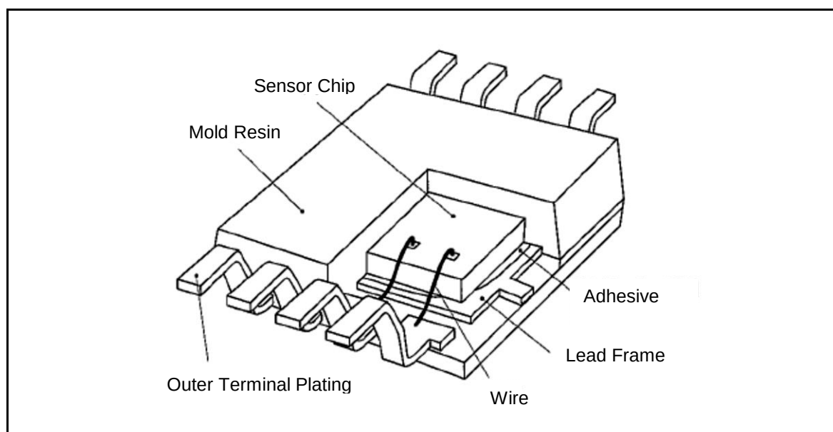
Figure 4-4 Internal Structure
