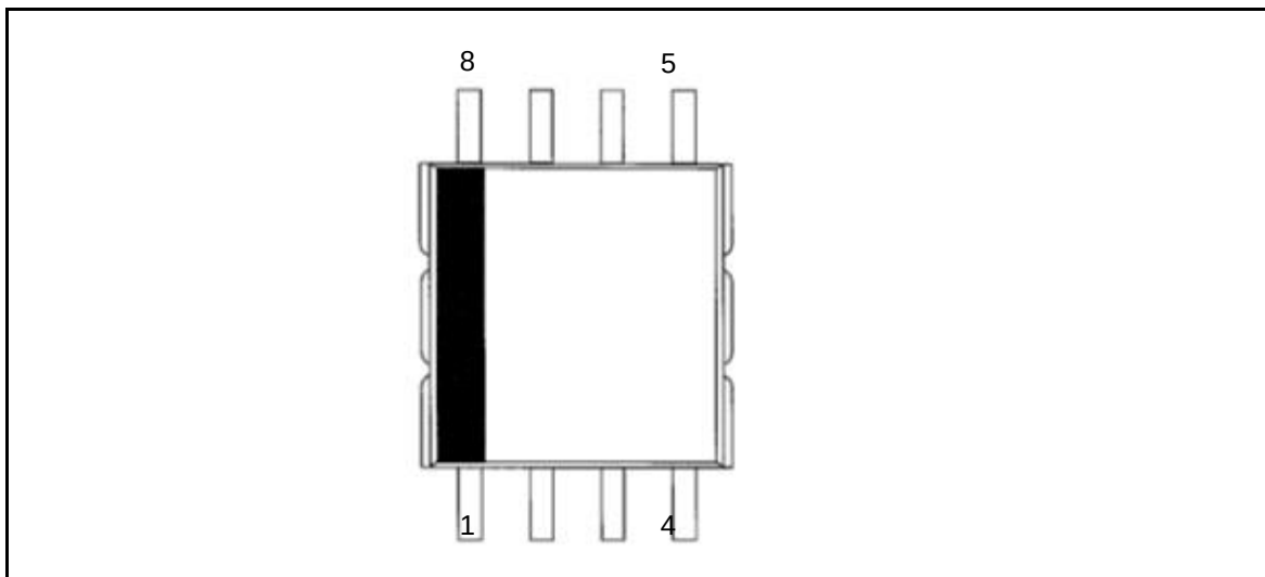
Figure 2-1 Pin Configuration
