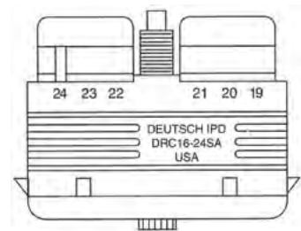
Standard Plug
