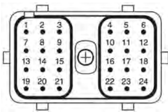
In-line Receptacle
