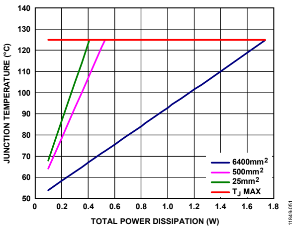
Figure 54. LFCSP, T A = 85°C
