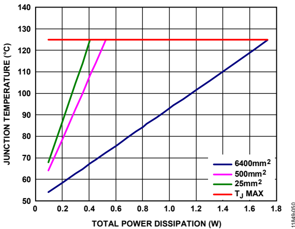
Figure 53. LFCSP, T A = 50°C
