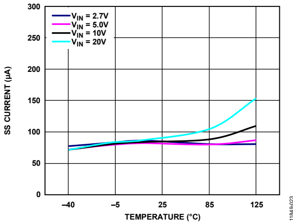
Figure 25. Soft Start (SS) Current vs. Temperature, Multiple Input Voltages, V_{OUT} = 5 V
