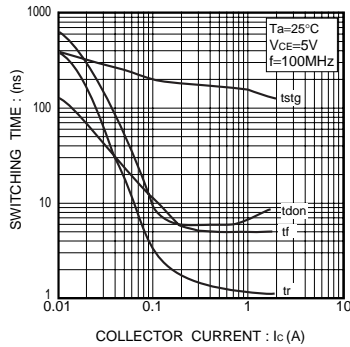
Fig.13 Switching time
