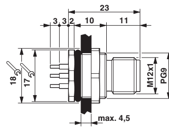
M12 flush-type connector
