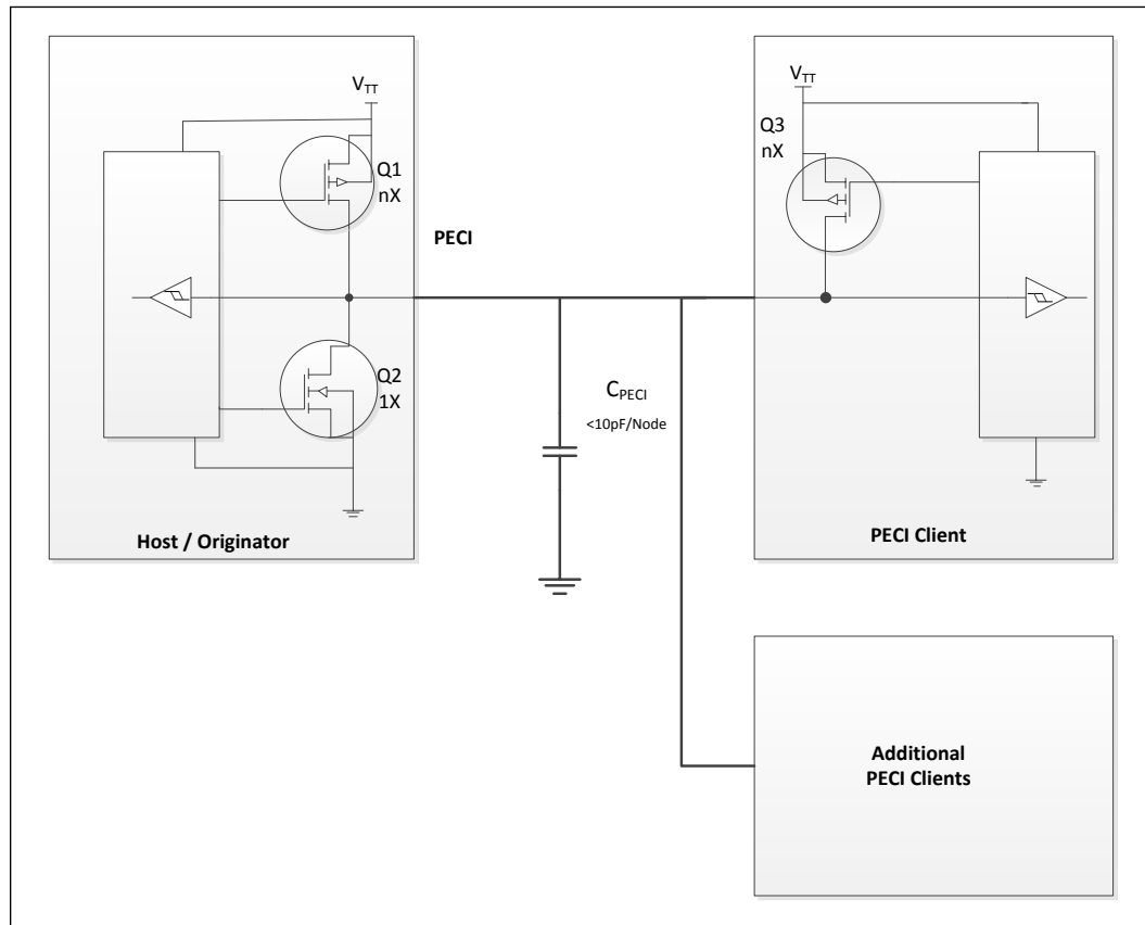
Figure 6. PEI Host-Clients Connection Example
