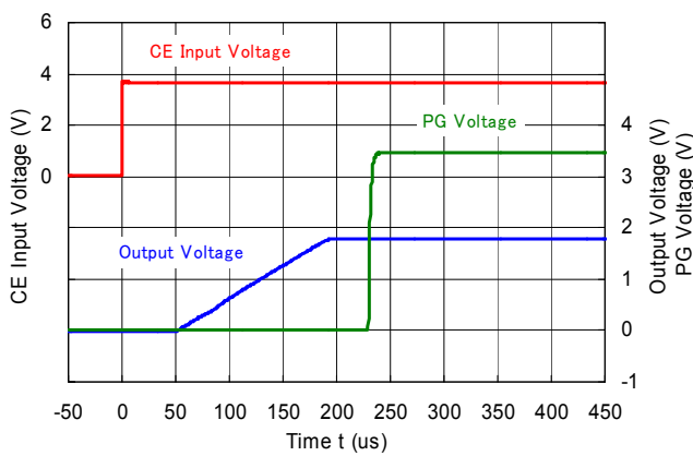
RP506K V_{OUT} = 1.8 V TSS = Open
