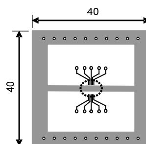
Standard Test Land Pattern
