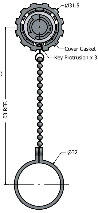
Protective Cover Bayonet Locking Style (Zinc Die-Cast Version)
