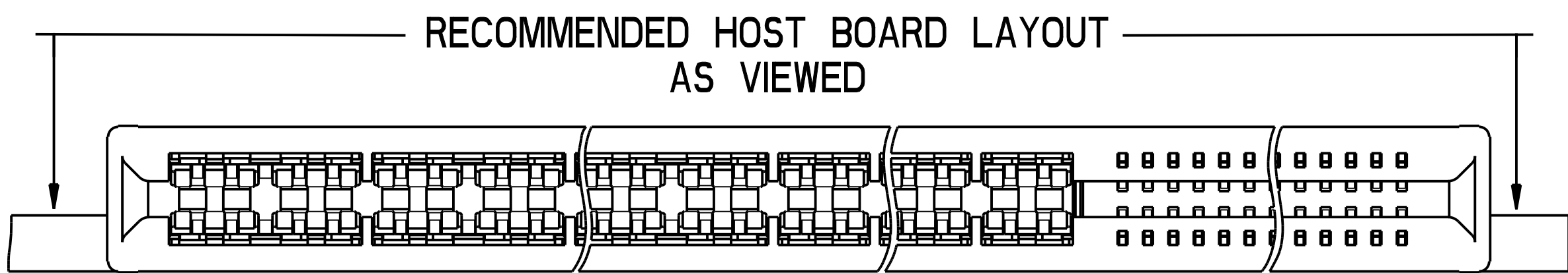
RECOMMENDED HOST BOARD LAYOUT TOLERANCE \pm 0.05
