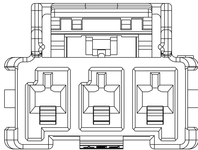
1*3 POSITIONS
