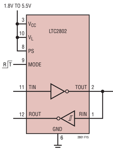
Figure 15. Half-Duplex on Single Line, Separate R OUT , T IN
