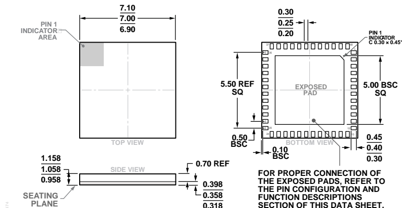
Figure 45. 48-Terminal Land Grid Array Package (LGA) (CC-48-4) Dimensions shown in millimeters
