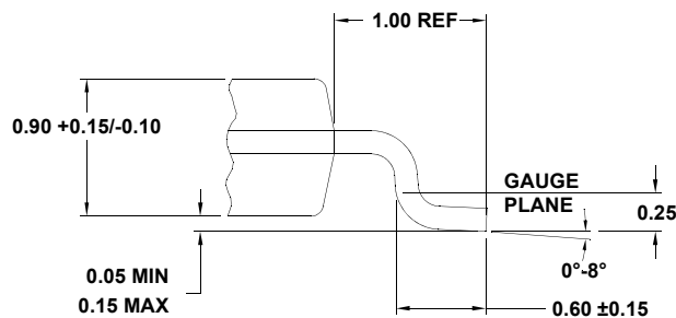
DETAIL "X"
