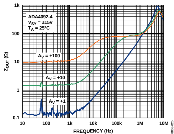
Figure 25. Output Impedance vs. Frequency, 30 V
