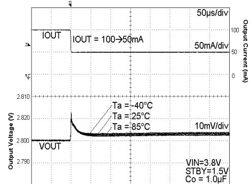
Fig. 55 Load Response
