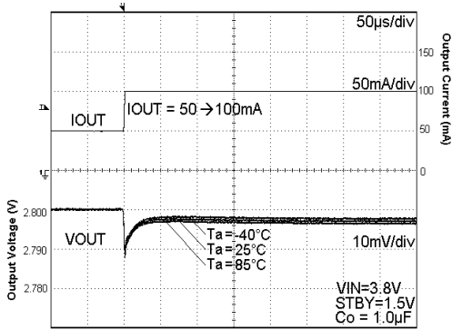
Fig. 54 Load Response
