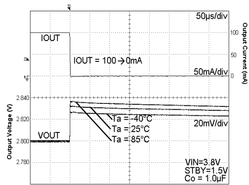
Fig. 53 Load Response
