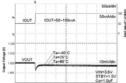
Fig. 112 Load Response
