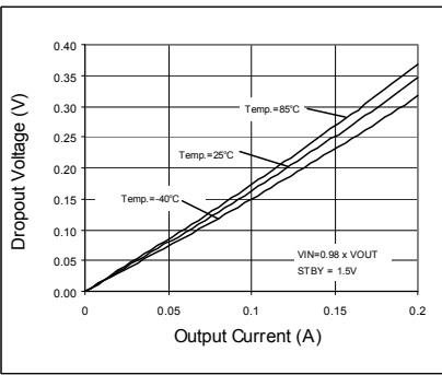
Fig. 43 Dropout Voltage
