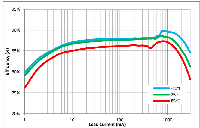
Figure 7. Efficiency vs. Load Current and Temperature, V_{IN}=3.6\text{ V} , V_{OUT}=1.15625\text{ V}
