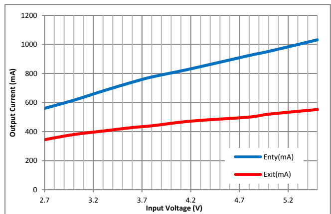
Figure 9. PWM Entry / Exit Level vs. Input Voltage, V_{OUT}=1.15625\text{ V}
