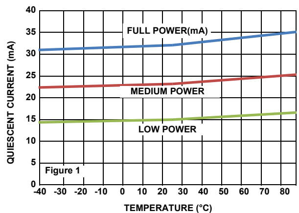
FIGURE 32. QUIESCIENT CURRENT vs TEMPERATURE
