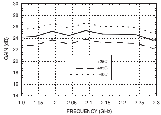
Gain vs. Temperature @ 2100 MHz
