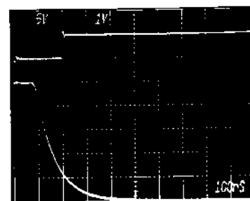
EXPANDED DAC OUTPUT SETTLING TIME NEGATIVE TRANSITION
