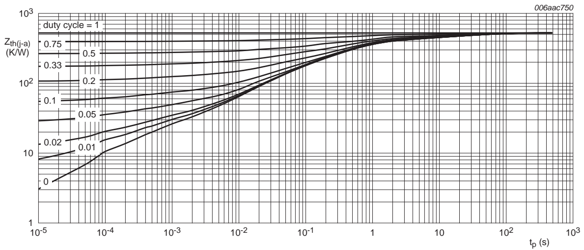
Fig 3. Per transistor: Transient thermal impedance from junction to ambient as a function of pulse duration for PUMB15 (SOT363); typical values
