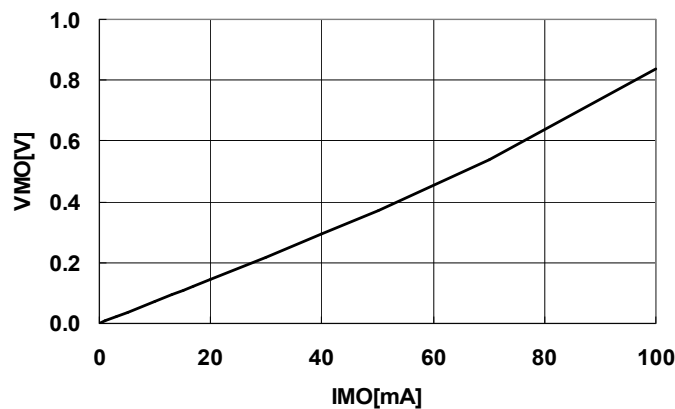
IMO VS. VMO VDD=5V T_a=25[^\circ\text{C}]
