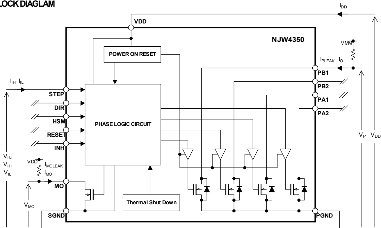
Fig.2 Block Diagram
