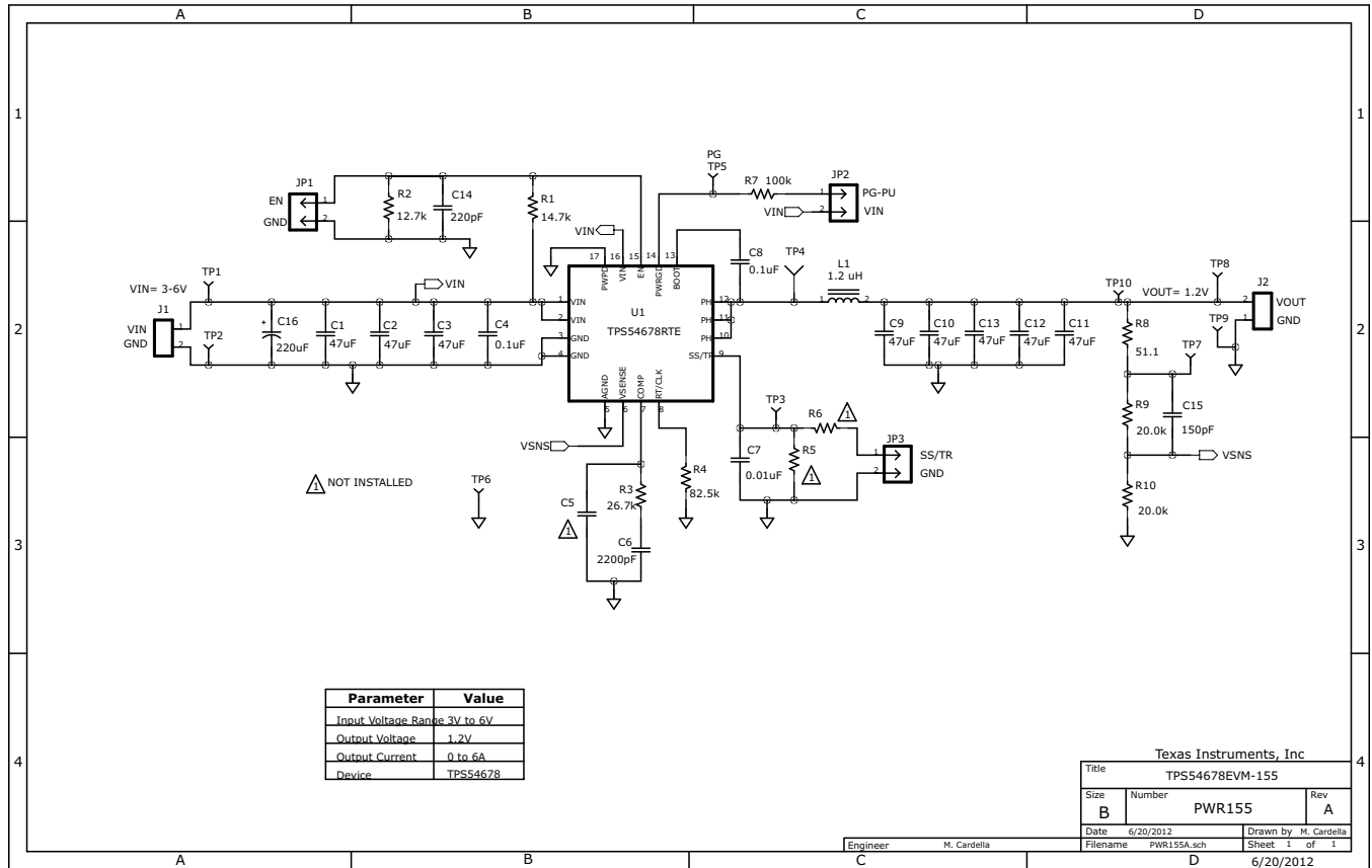
Figure 23. TPS54678EVM-155 Schematic
