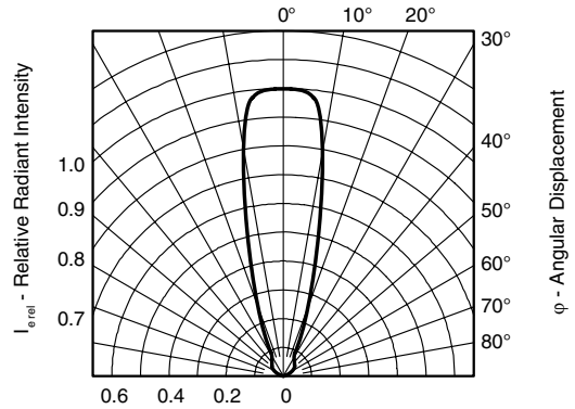
94 8008 Fig. 10 - Relative Radiant Intensity vs. Angular Displacement
