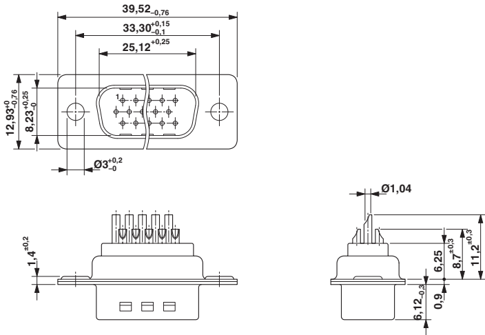
Dimensioned drawing
