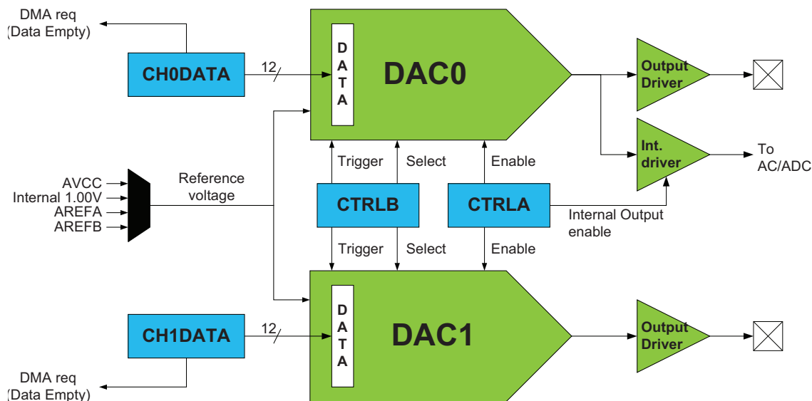
Figure 30-1. DAC overview.
