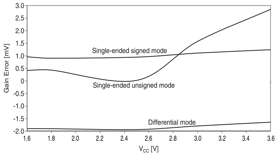
Figure 38-42. Gain error vs. V_{CC} .
