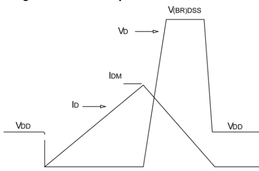
Figure 20: Unclamped inductive waveform
