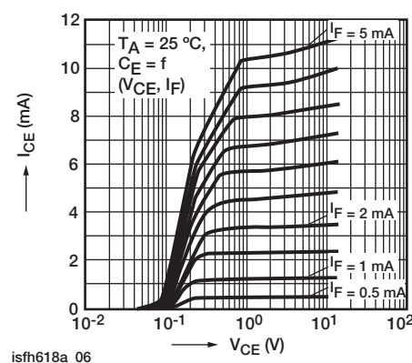
Fig. 8 - Output Characteristics
