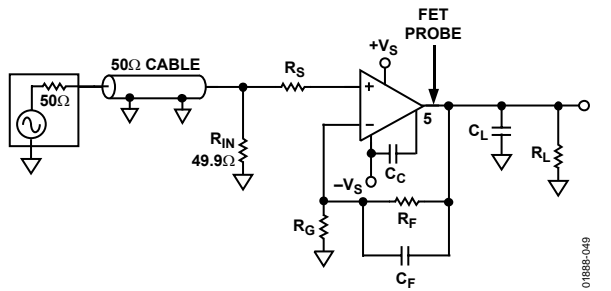
Figure 49. Noninverting Gain and FET Probe
